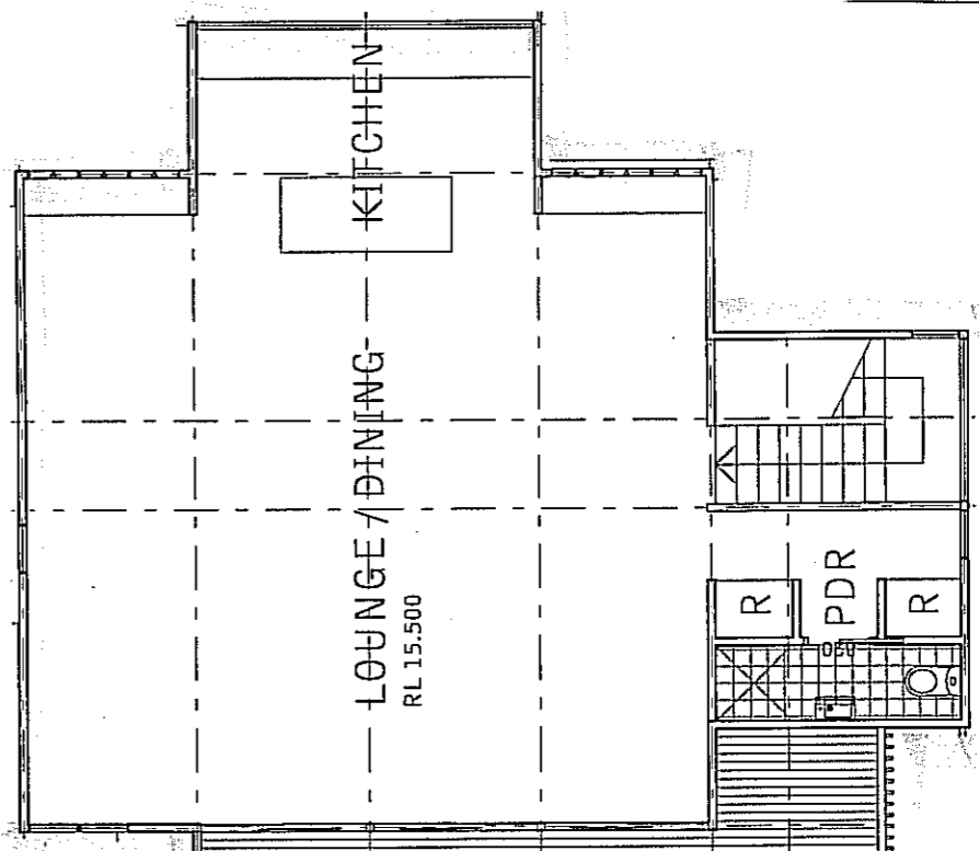
House ONE (3 Bedroom Option) Upper Floor PLAN
